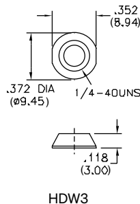
Dress Nut
