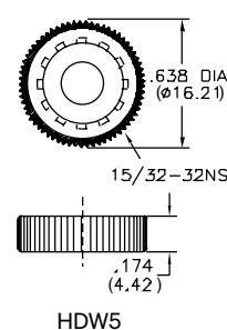
Knurled Nut (Sealed)
