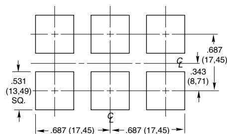
Figure 1 Panel Mount Cutout Diagram
